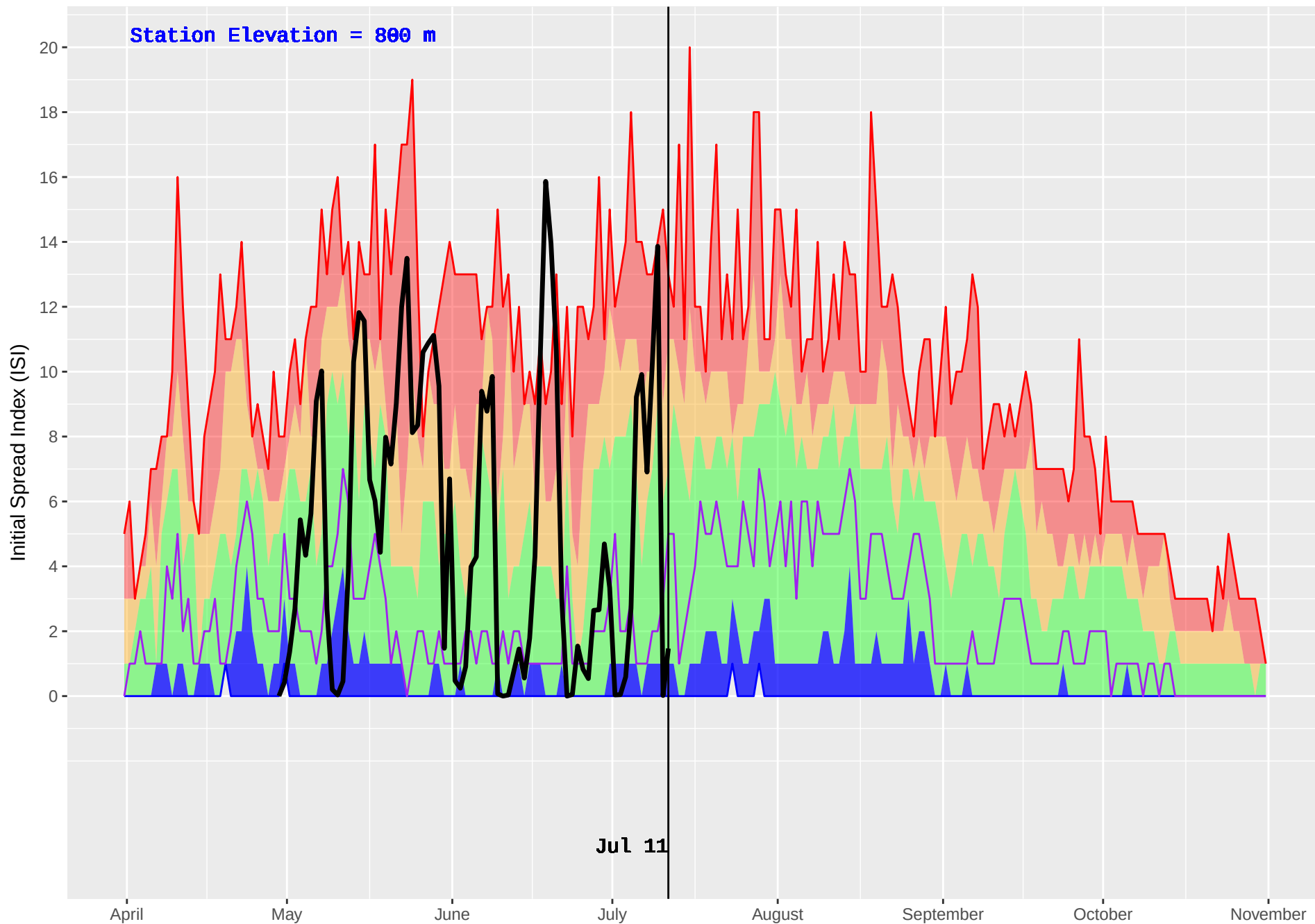
GOLD HILL (379) : Historical (1979–2016) and Current (2018) Noon Initial Spread Index (ISI)
